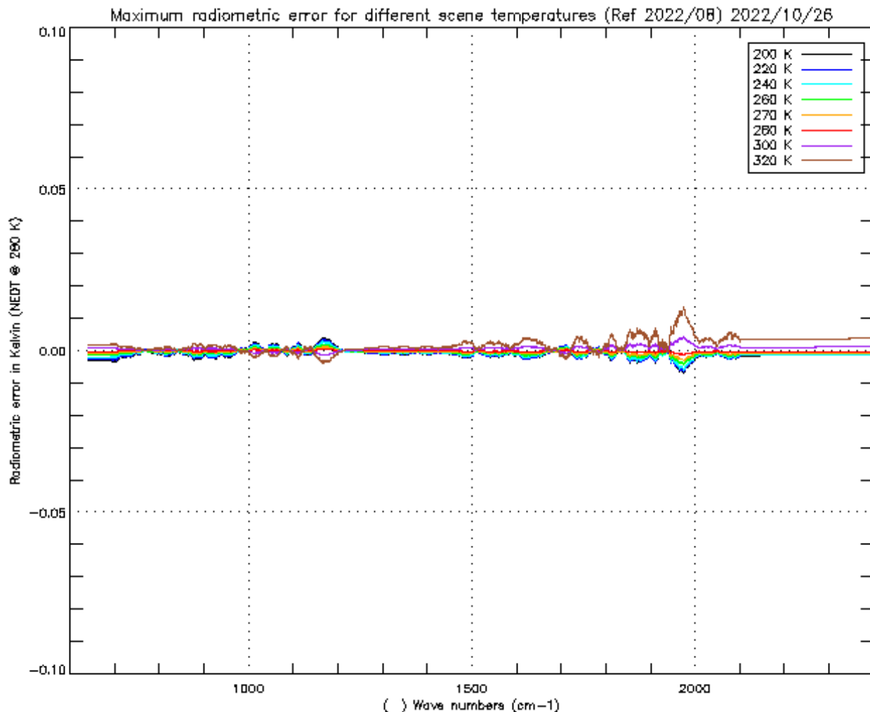
Figure 23 : Radiometric calibration error due to scan mirror reflectivity dependency with viewing angle Maximum effect on SN1 for different scene temperature. Done with the period August 22 / October 22
