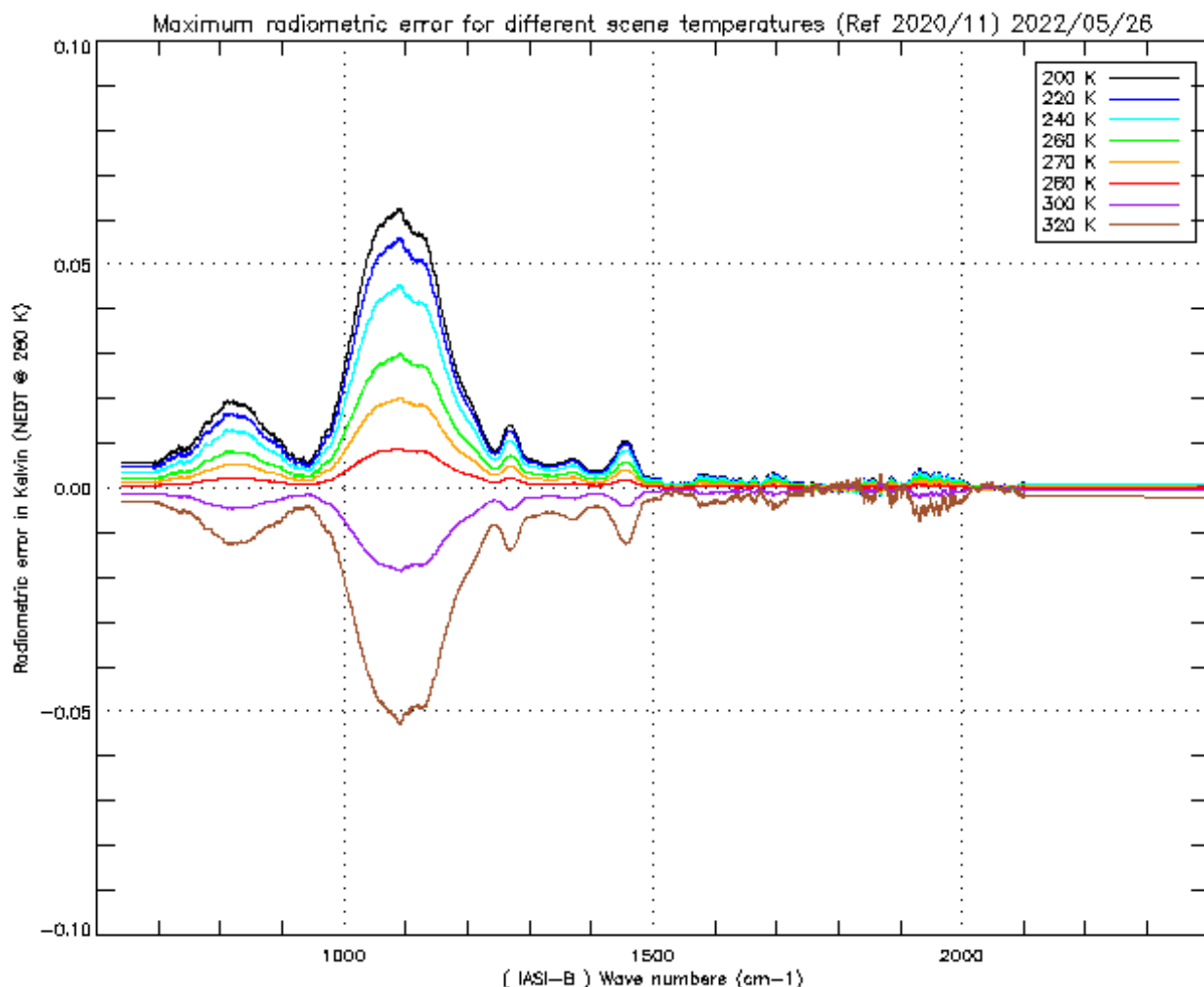
Figure 23 : Radiometric calibration error due to scan mirror reflectivity dependency with viewing angle Maximum effect on SN1 for different scene temperature. Done with the period November 20 / May 22
