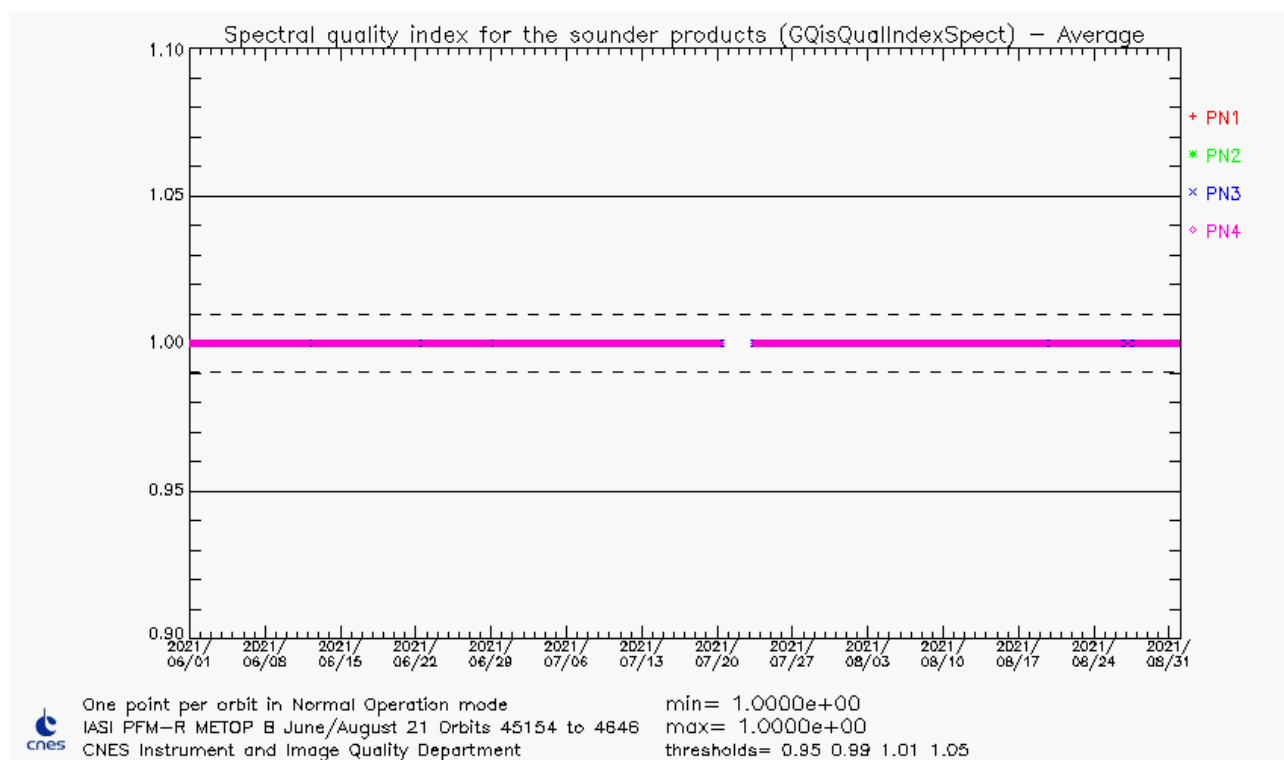
Figure 17 : GQisQualIndexSpect average (L1 data index for spectral calibration quality)
