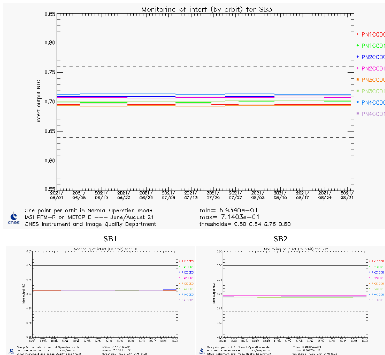
Figure 29 : Contrast Monitoring
