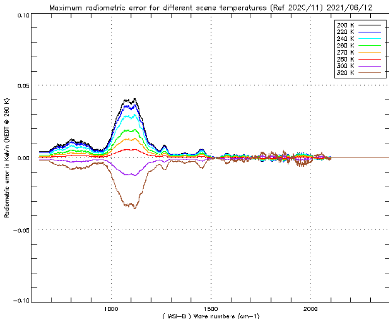
Figure 23 : Radiometric calibration error due to scan mirror reflectivity dependency with viewing angle Maximum effect on SN1 for different scene temperature. Done with the period November 20 / June 21
