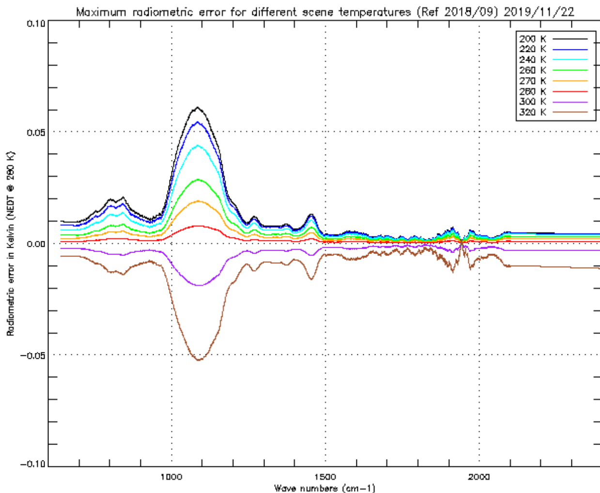
Figure 23 : Radiometric calibration error due to scan mirror reflectivity dependency with viewing angle Maximum effect on SN1 for different scene temperature. Done with the period September 18 / November 19
