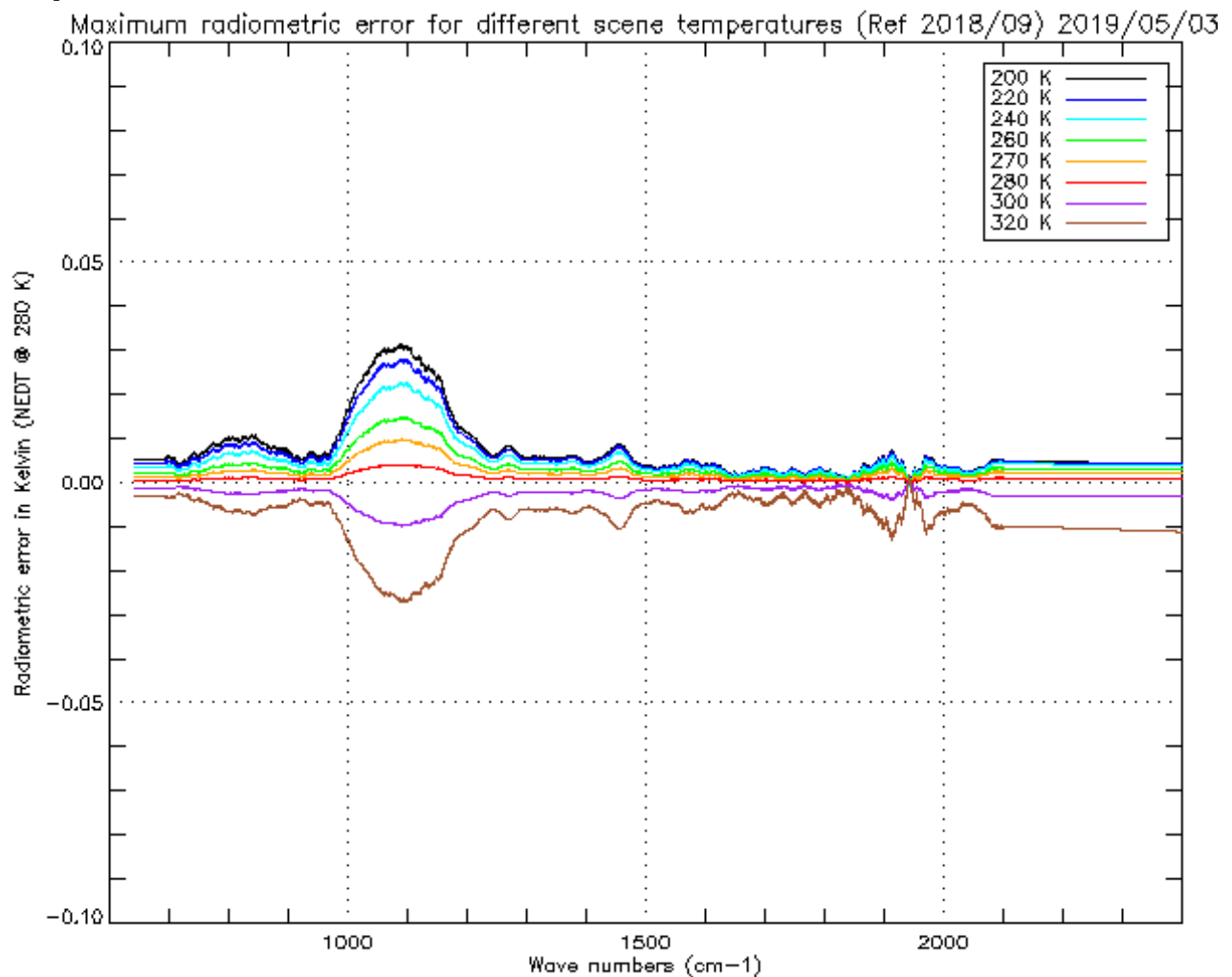
Figure 23 : Radiometric calibration error due to scan mirror reflectivity dependency with viewing angle Maximum effect on SN1 for different scene temperature. Done with the period September 18 / May 19
