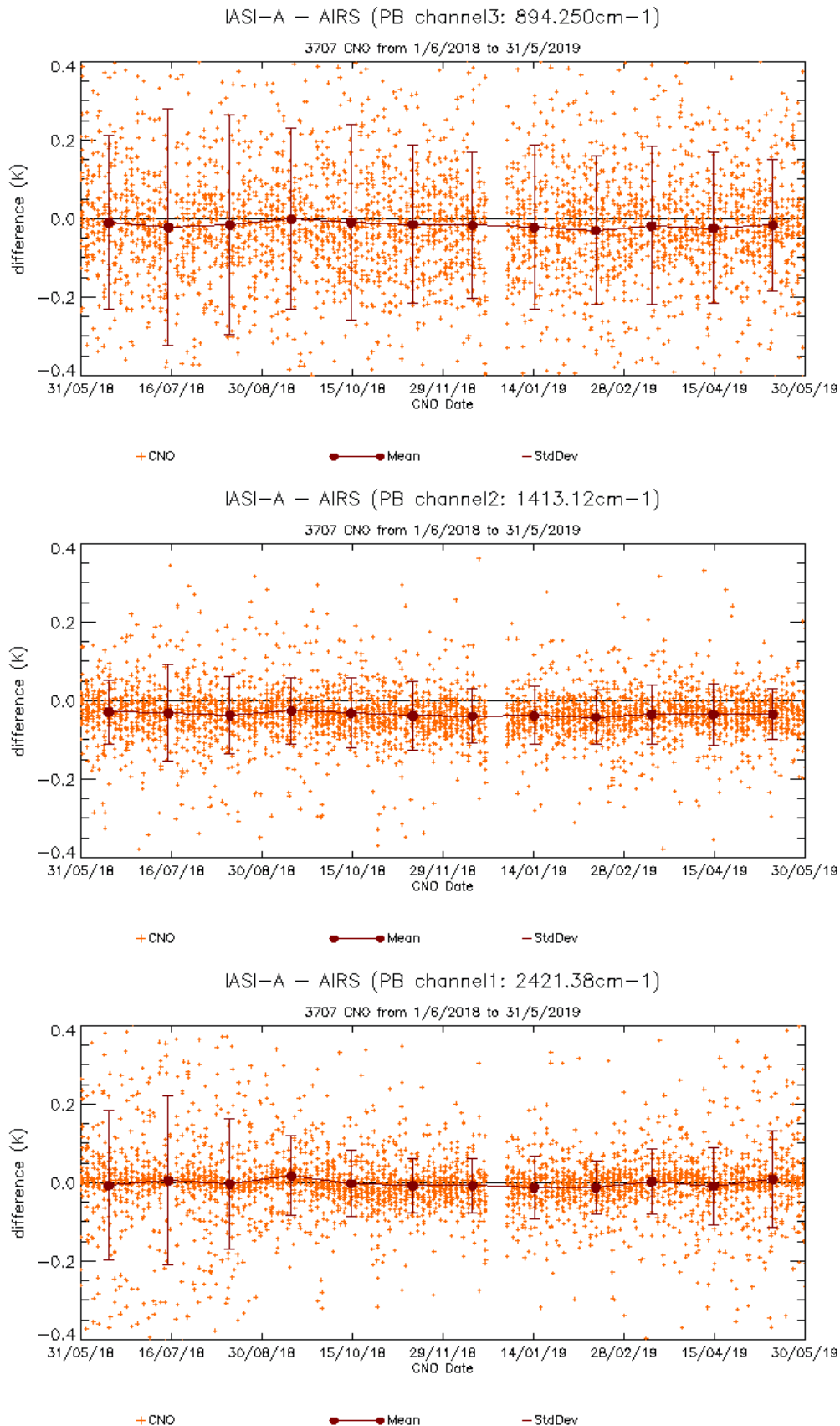
Figure 39 : Temporal evolution of the differences IASI-A – AIRS in brightness temperature over the approximate three IASI bands, with monthly means
