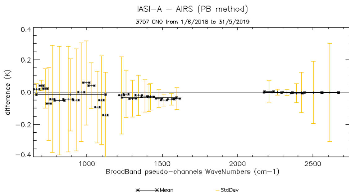
Figure 38 : Mean (black curve) and standard deviation (yellow) of the difference in brightness temperature IASI-A – AIRS.
