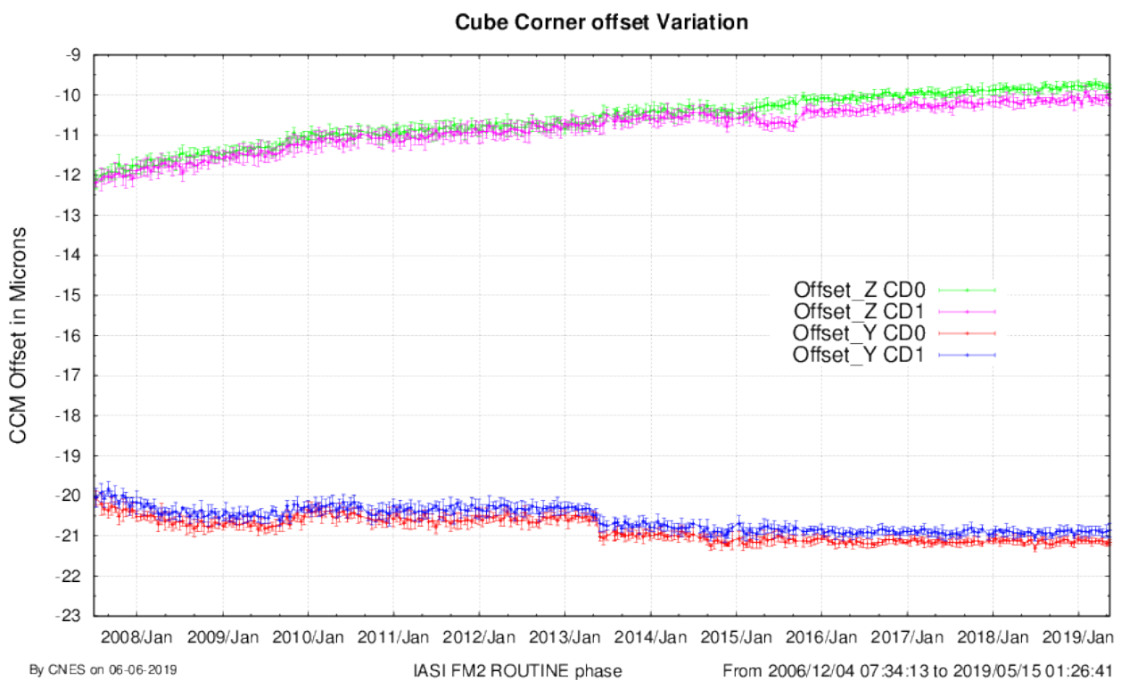
Figure 34 : Cube Corner offset variation
