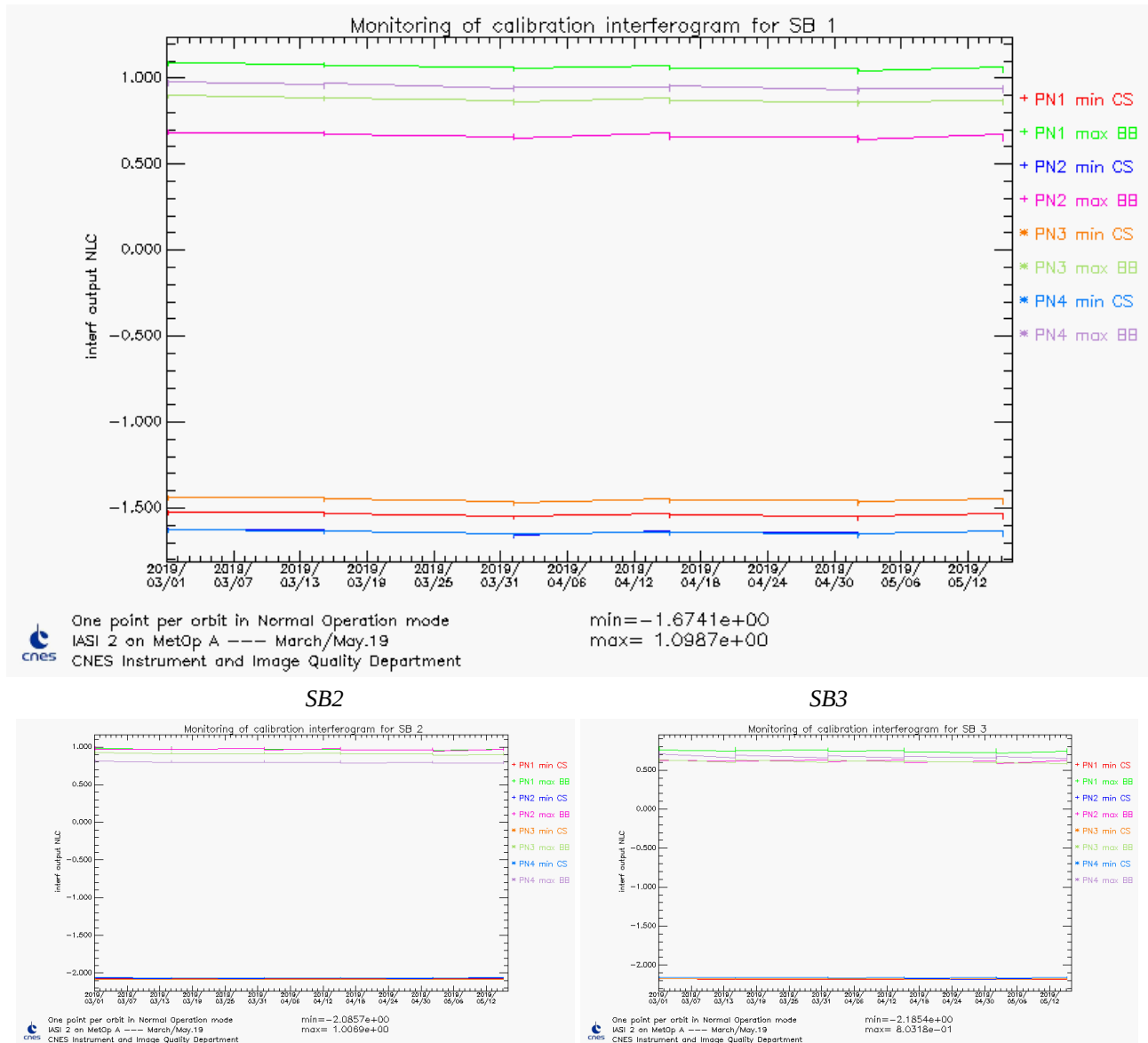
Figure 31 : Monitoring of detection chain margins
