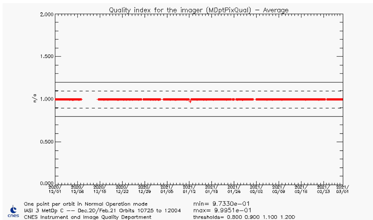
Figure 20 : MDptPixQual average (L1 quality index for IASI integrated imager, fraction of not dead pixels)
