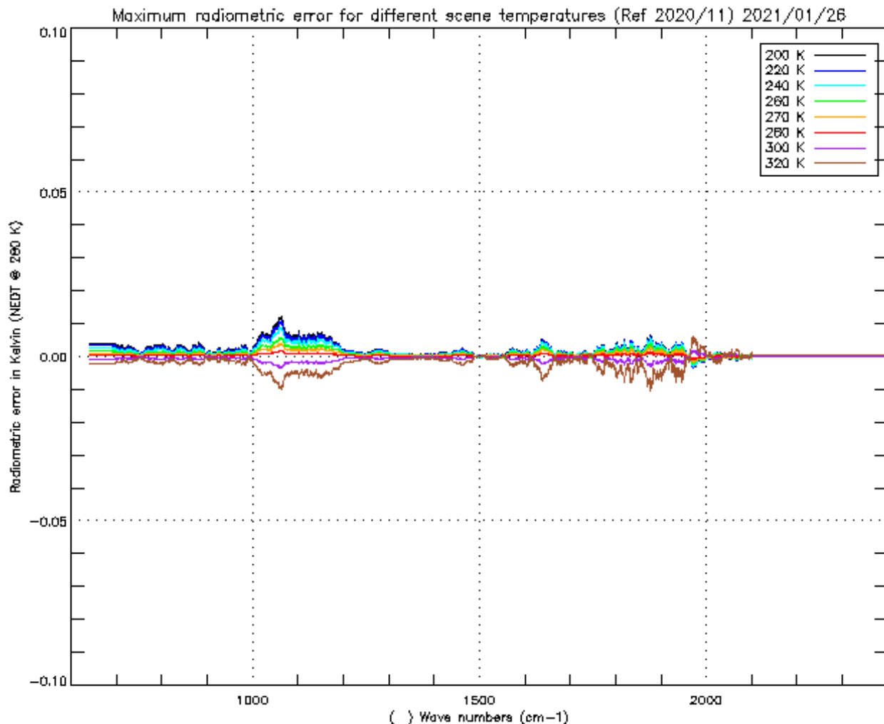
Figure 23 : Radiometric calibration error due to scan mirror reflectivity dependency with viewing angle Maximum effect on SN1 for different scene temperature. Done with the period November 20 /January 21
