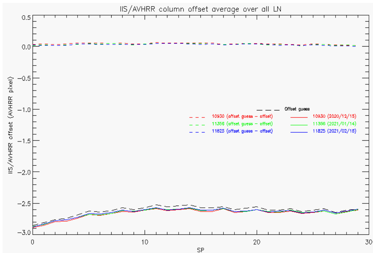
Figure 36 : Column offset (black) guess vs. column offset averaged over all lines (LN) as a function of the scan position (SP=SN), and orbit number (along track IIS/AVHRR offset)
