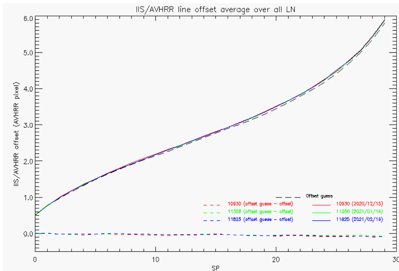
Figure 37 : Line offset guess (black) vs. line offset averaged over all lines (LN) as a function of the scan position (SP=SN), and the orbit number (across track IIS/AVHRR offset)
