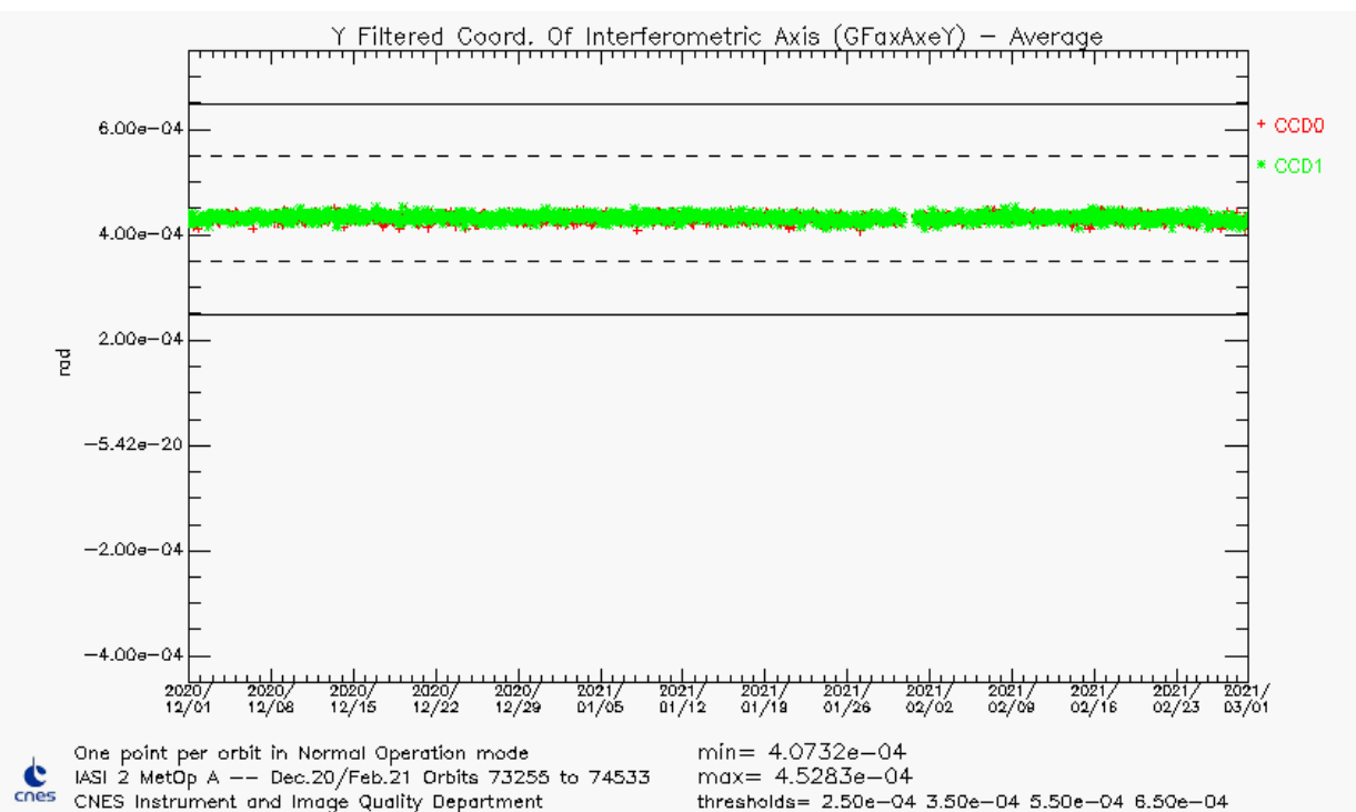
Figure 32 : GFAxAxisY average (Y filtered coordinates of sounder interferometric axis)
