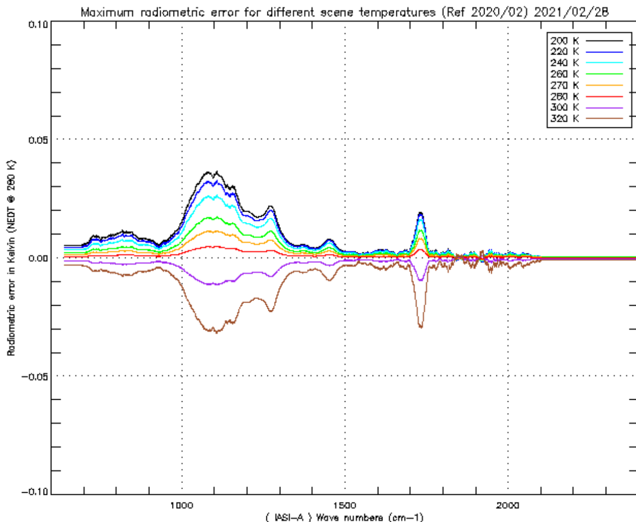
Figure 23 : Radiometric calibration error due to scan mirror reflectivity dependency with viewing angle Maximum effect on SN1 for different scene temperature. Done with the period February 20 / February 2021
