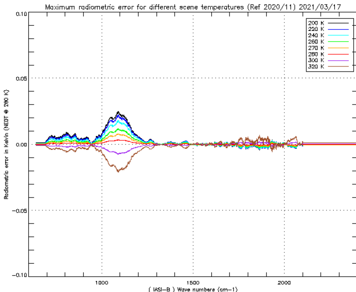
Figure 23 : Radiometric calibration error due to scan mirror reflectivity dependency with viewing angle Maximum effect on SN1 for different scene temperature. Done with the period November 20 / March 21
