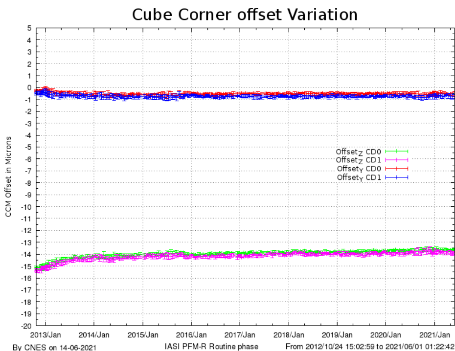
Figure 34 : Cube Corner offset variation
