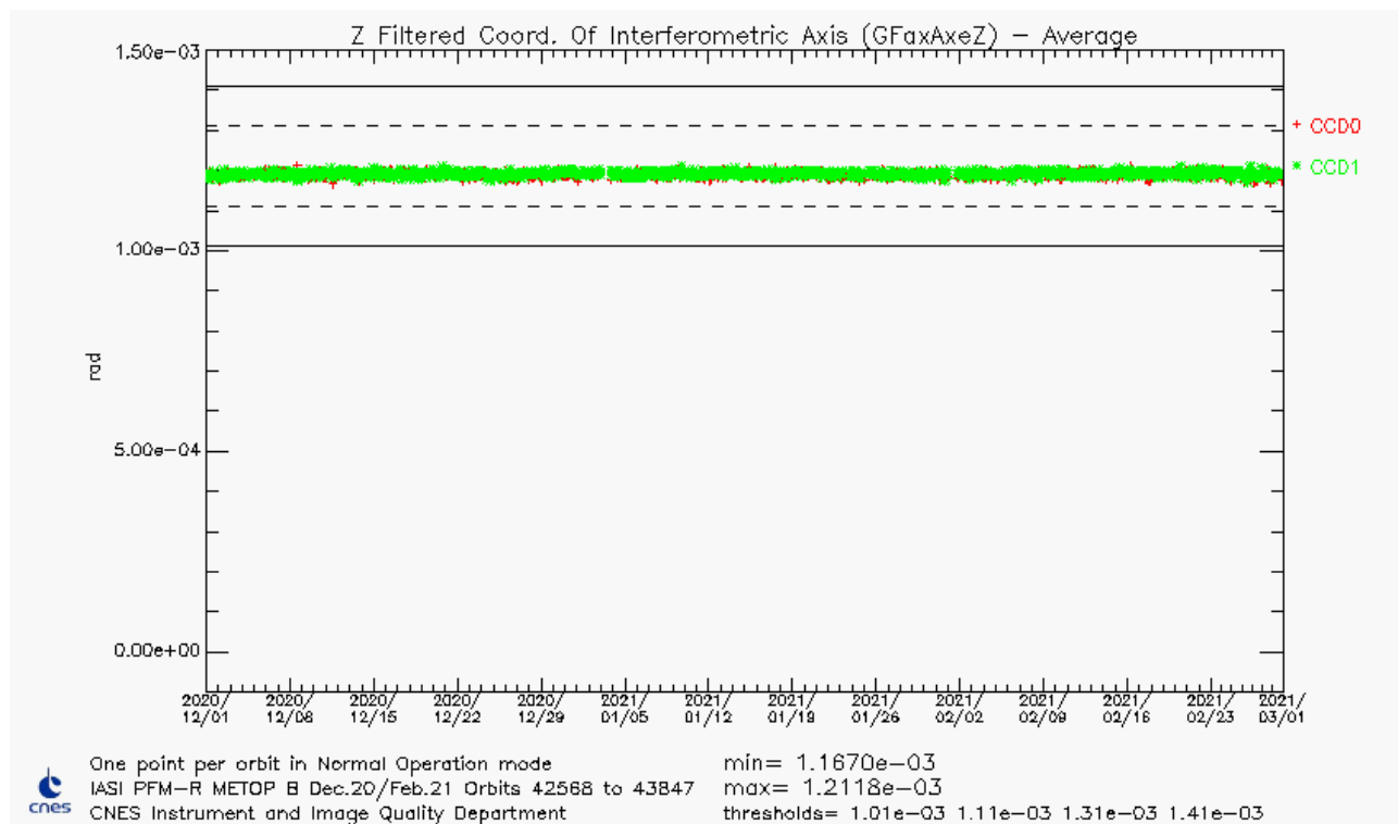
Figure 33 : GFAxAxisZ average (Z filtered coordinates of sounder interferometric axis)
