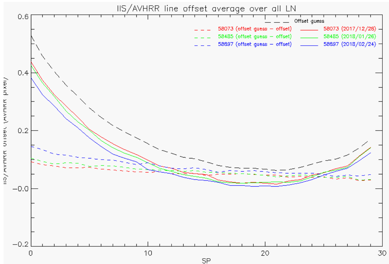
Figure 37 : Line offset guess (black) vs. line offset averaged over all lines (LN) as a function of the scan position (SP=SN), and the orbit number
