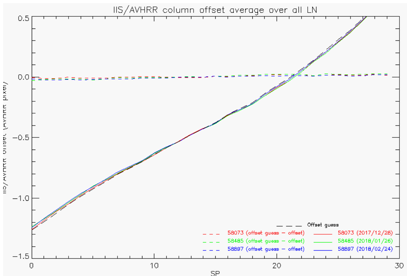
Figure 36 : Column offset (black) guess vs. column offset averaged over all lines (LN) as a function of the scan position (SP=SN), and orbit number
