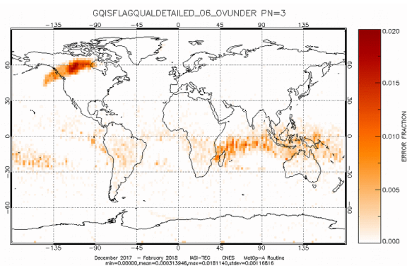
Figure 9 : IASI Overflows and Underflows spatial distribution (per pixel)
