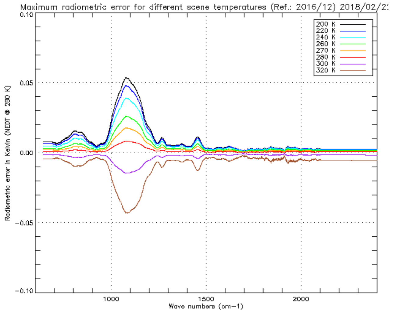
Figure 23 : Radiometric calibration error due to scan mirror reflectivity dependency with viewing angle Maximum effect on SN1 for different scene temperature. Done with the period February 17 / February 18
