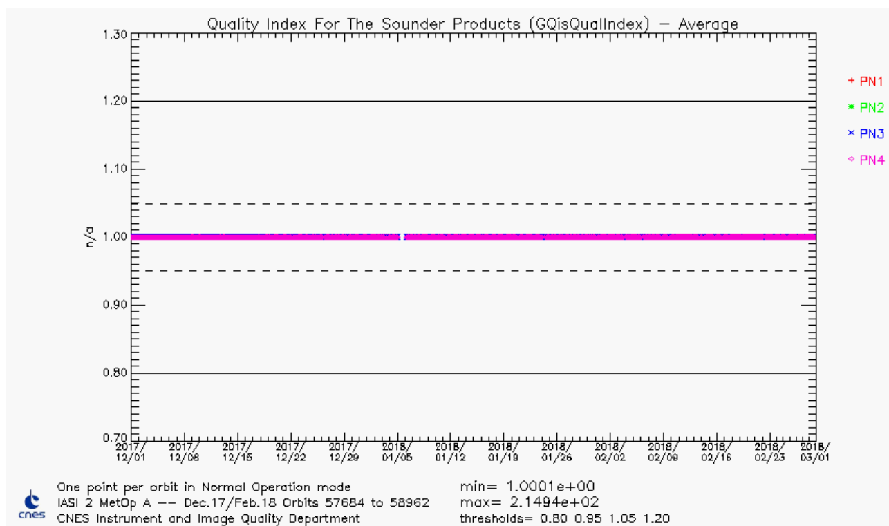
Figure 15 : GQisQualIndex average (L1 data quality index for IASI sounder)
