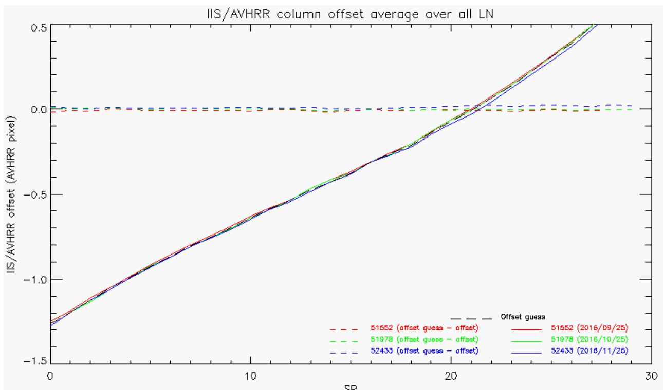
Figure 35 : Column offset (black) guess vs. column offset averaged over all lines (LN) as a function of the scan position (SP=SN), and orbit number
