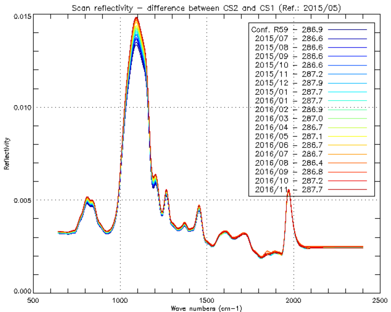
Figure 21 : Scan mirror reflectivity evolution
