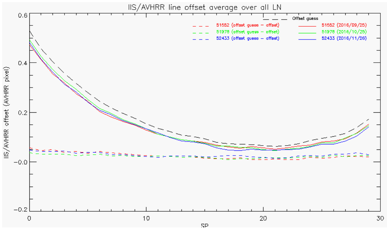
Figure 36 : Line offset guess (black) vs. line offset averaged over all lines (LN) as a function of the scan position (SP=SN), and the orbit number
