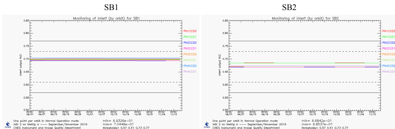
Figure 28 : Contrast Monitoring
