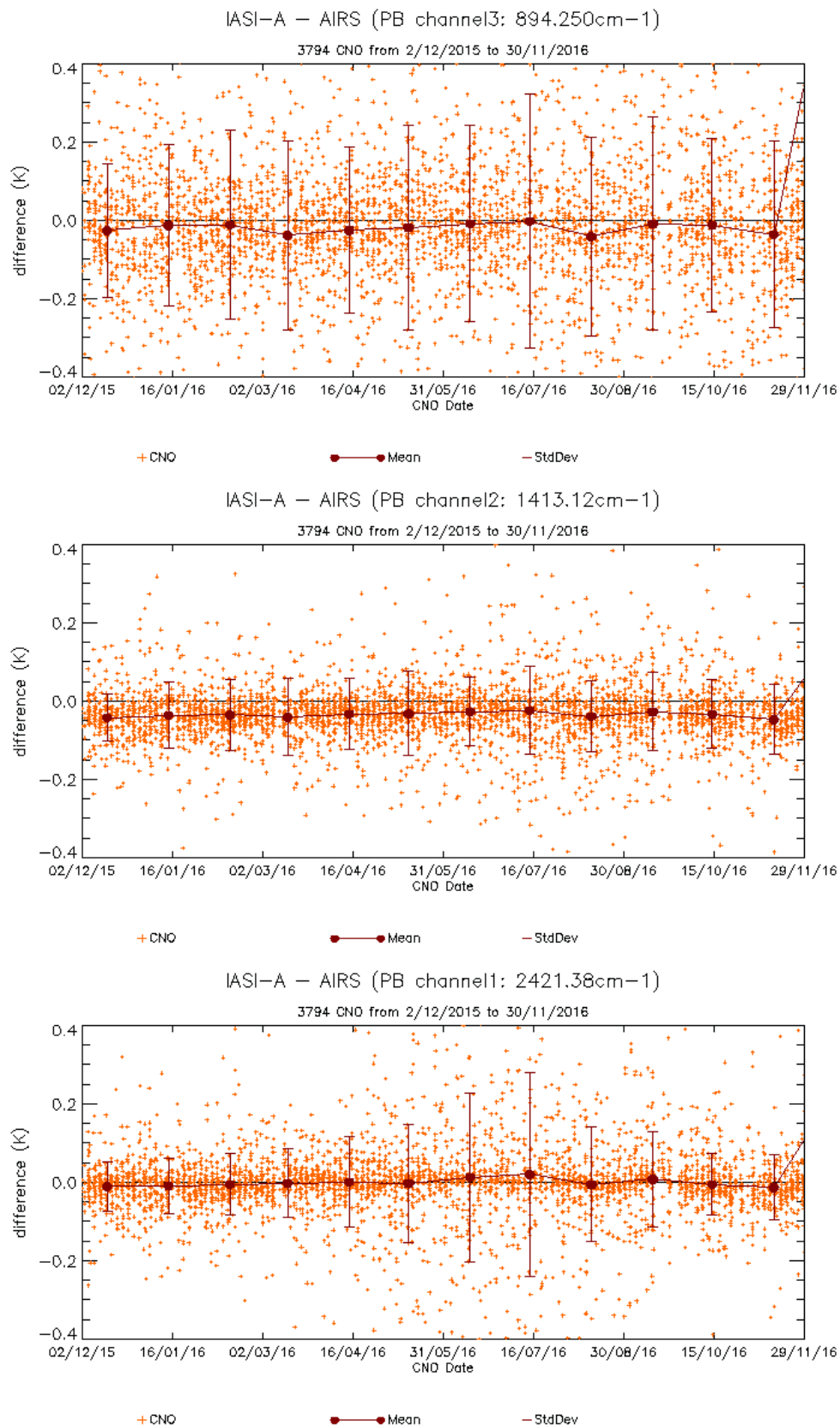
Figure 40 : Temporal evolution of the differences IASI-A – AIRS in brightness temperature over the approximate three IASI bands, with monthly means
