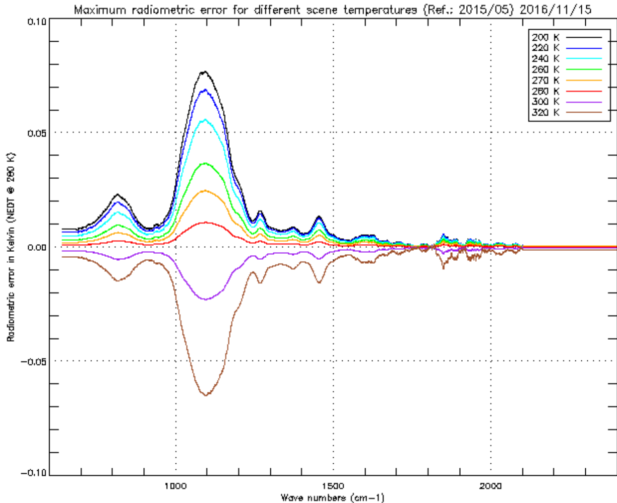
Figure 22 : Radiometric calibration error due to scan mirror reflectivity dependency with viewing angle Maximum effect on SN1 for different scene temperature. Done with the period May 15/ November 16
