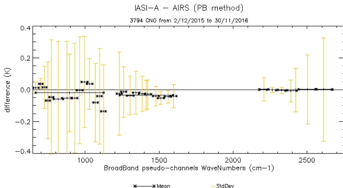
Figure 39 : Mean (black curve) and standard deviation (yellow) of the difference in brightness temperature IASI-A - AIRS.
