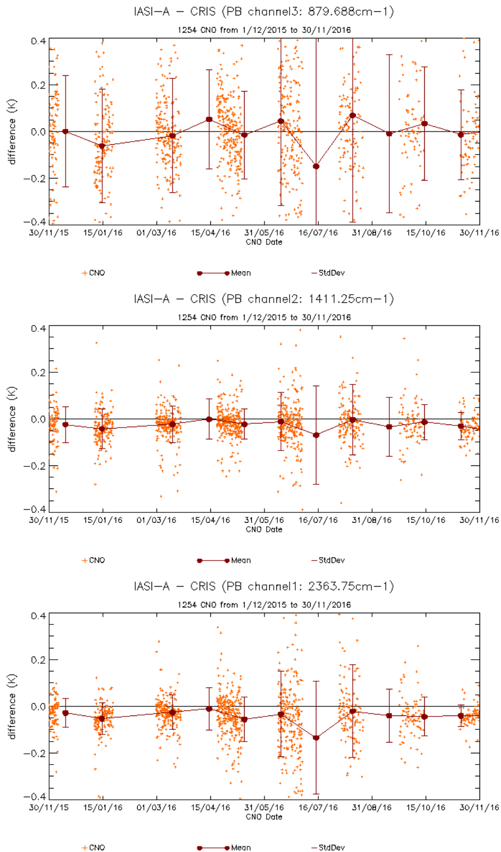
Figure 38 : Temporal evolution of the differences IASI-A – CRIS in brightness temperature over the approximate three IASI bands, with monthly means
