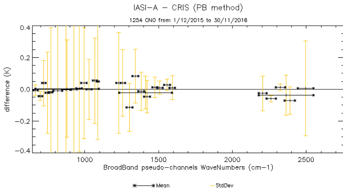
Figure 37 : Mean (black curve) and standard deviation (yellow) of the difference in brightness temperature IASI-A – CRIS
