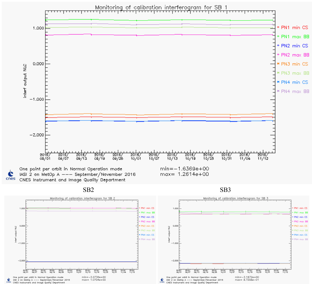
Figure 30 : Monitoring of detection chain margins
