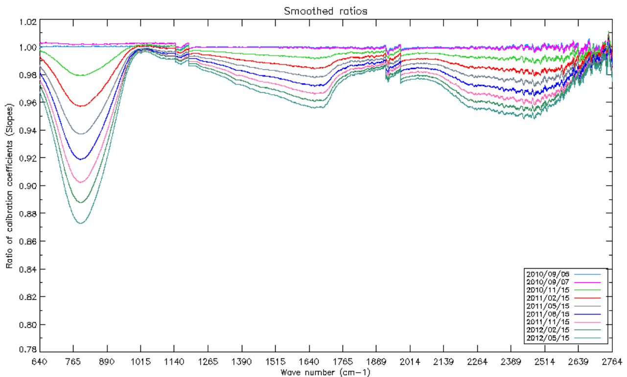
Figure 23 : Ratio of calibration coefficient slopes as a function of wave number and time after the second decontamination
