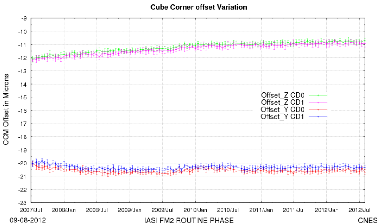
Figure 27 : Cube Corner offset variation
