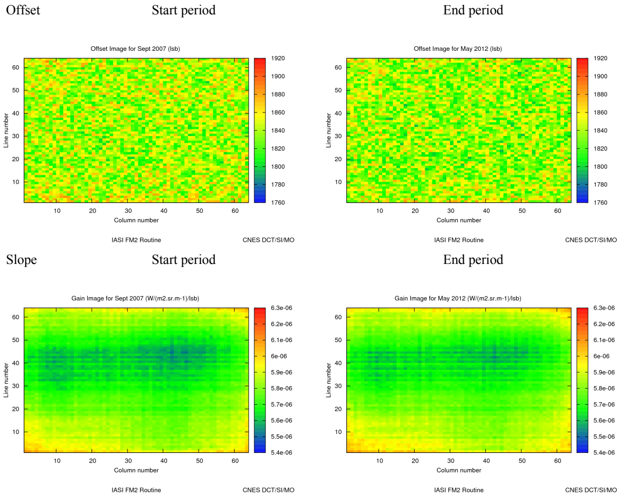
Figure 33 : Slope and offset coefficients matrix
