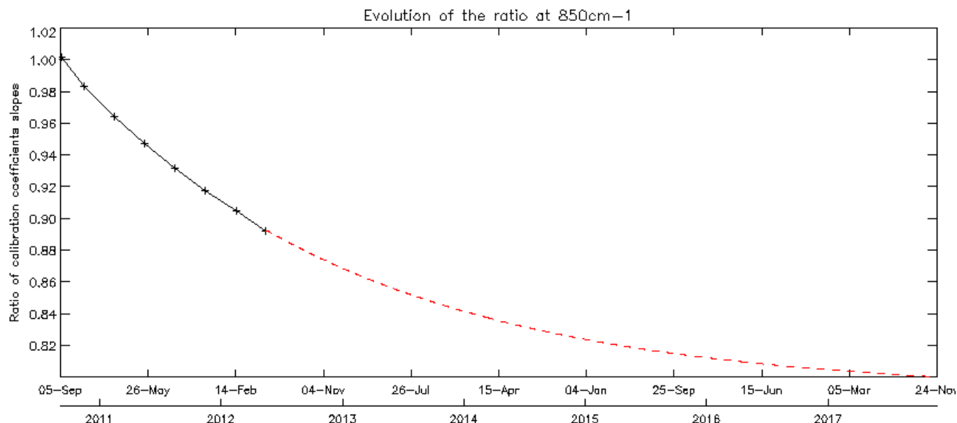
Figure 24 : Temporal evolution of calibration ratio coefficient slopes since the last decontamination.
