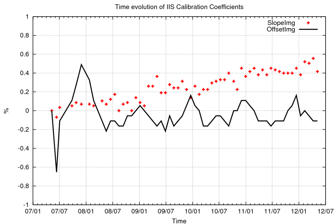
21-05-12 12:14 IASI FM2 ROUTINE CNES DCT/SIMO Figure 34 : Relative evolution in % of average of slope (red curve) and offset (black curve) coefficients
