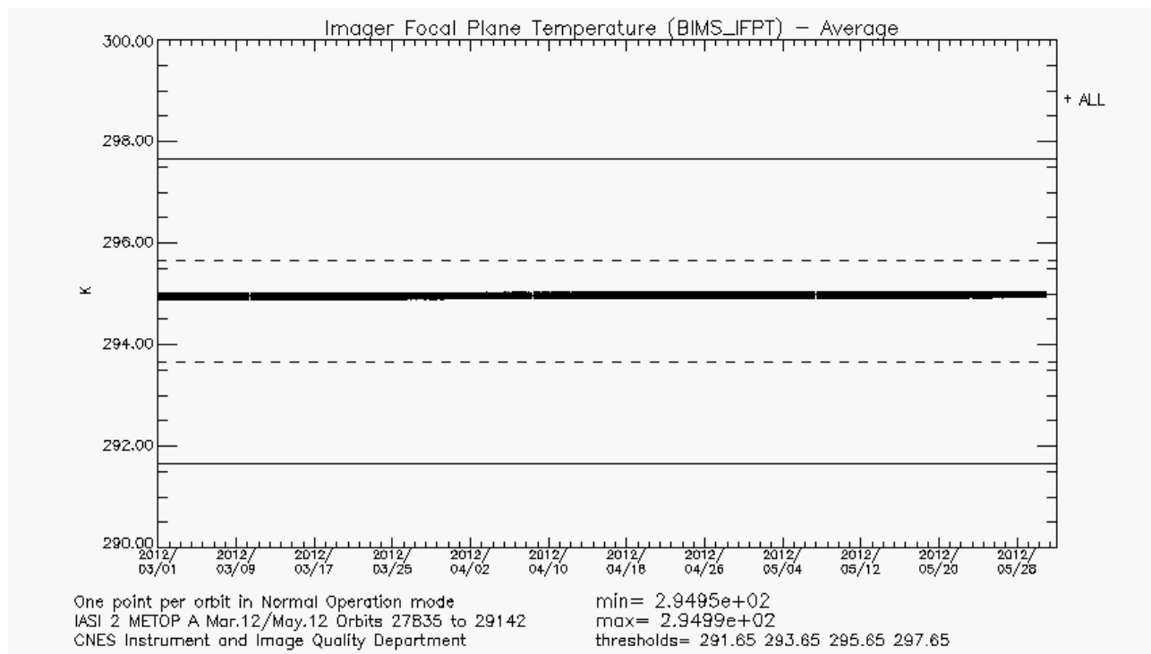
Figure 35 : IIS Focal Plane Temperature
