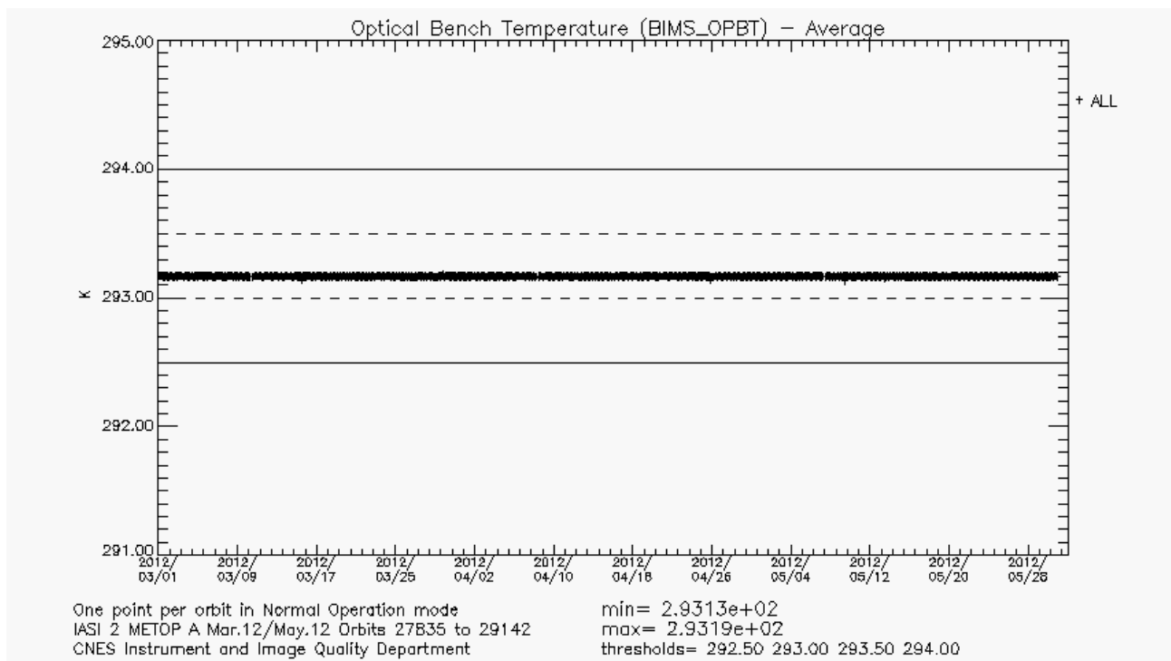
Figure 29 : Optical bench Temperature
