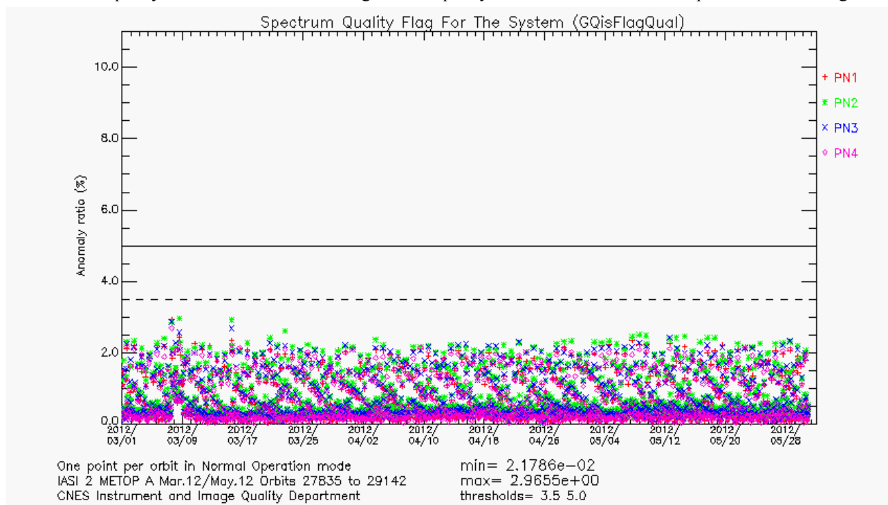
Figure 8 : IASI L1 data quality orbit average (% of bad by PN)
