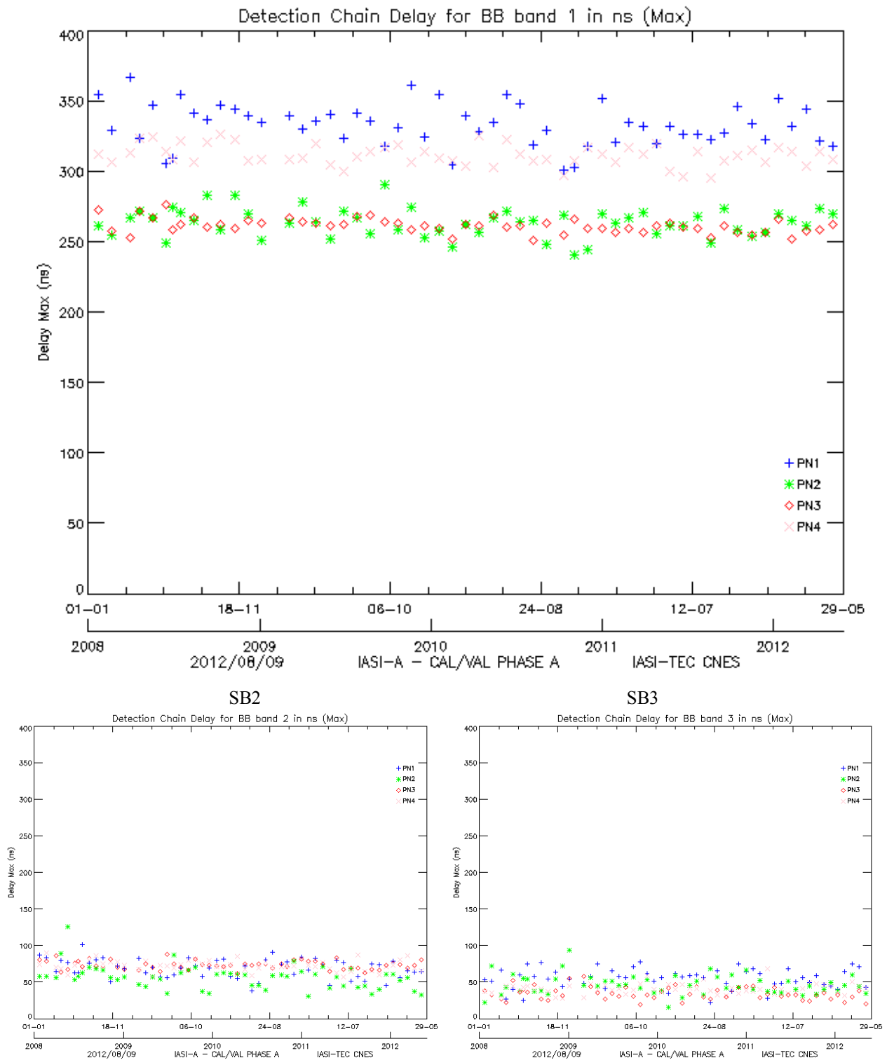
Figure 22 : Monitoring of detection chain maximum delays for all bands
