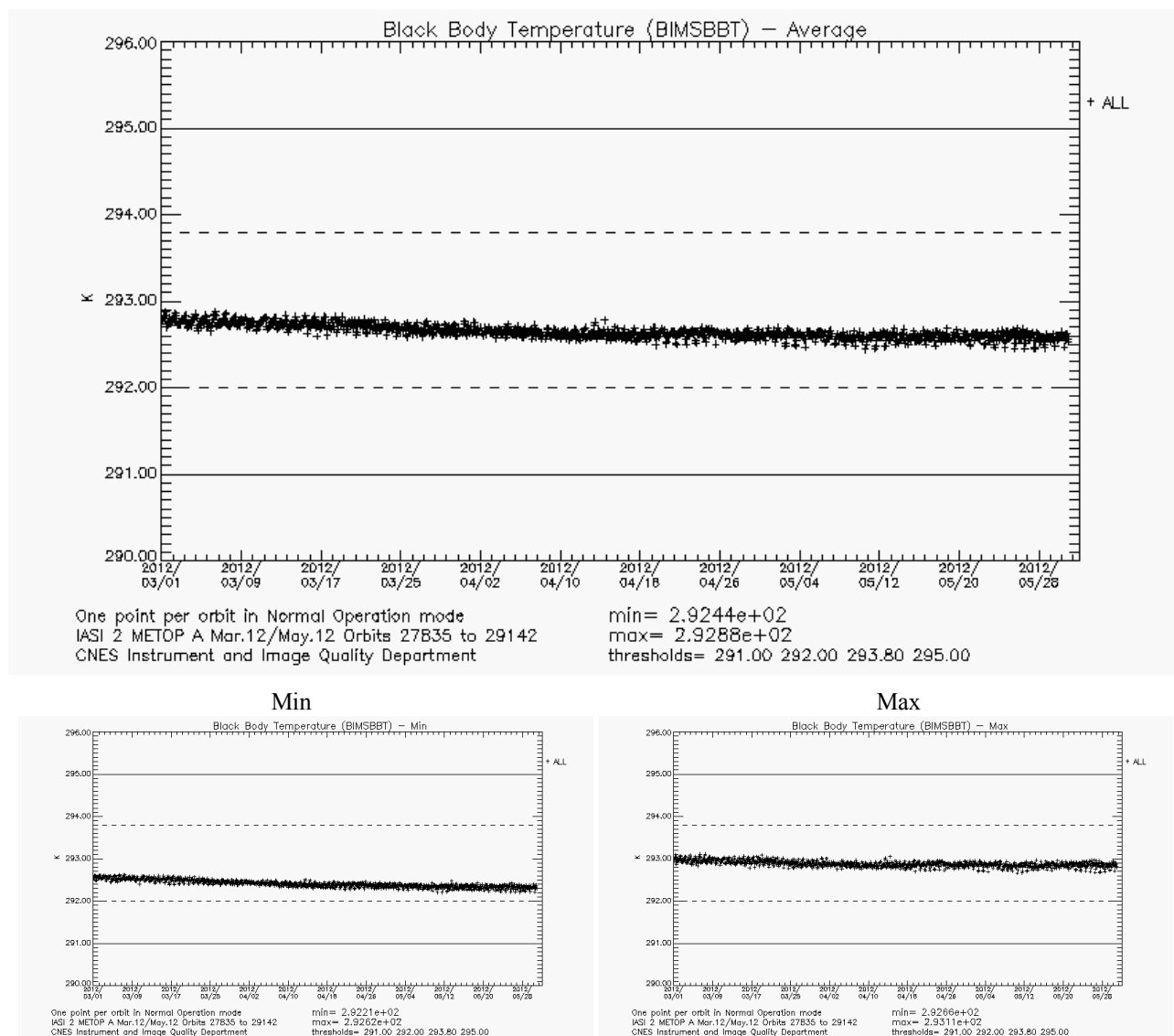
Figure 20 : Black Body Temperature
