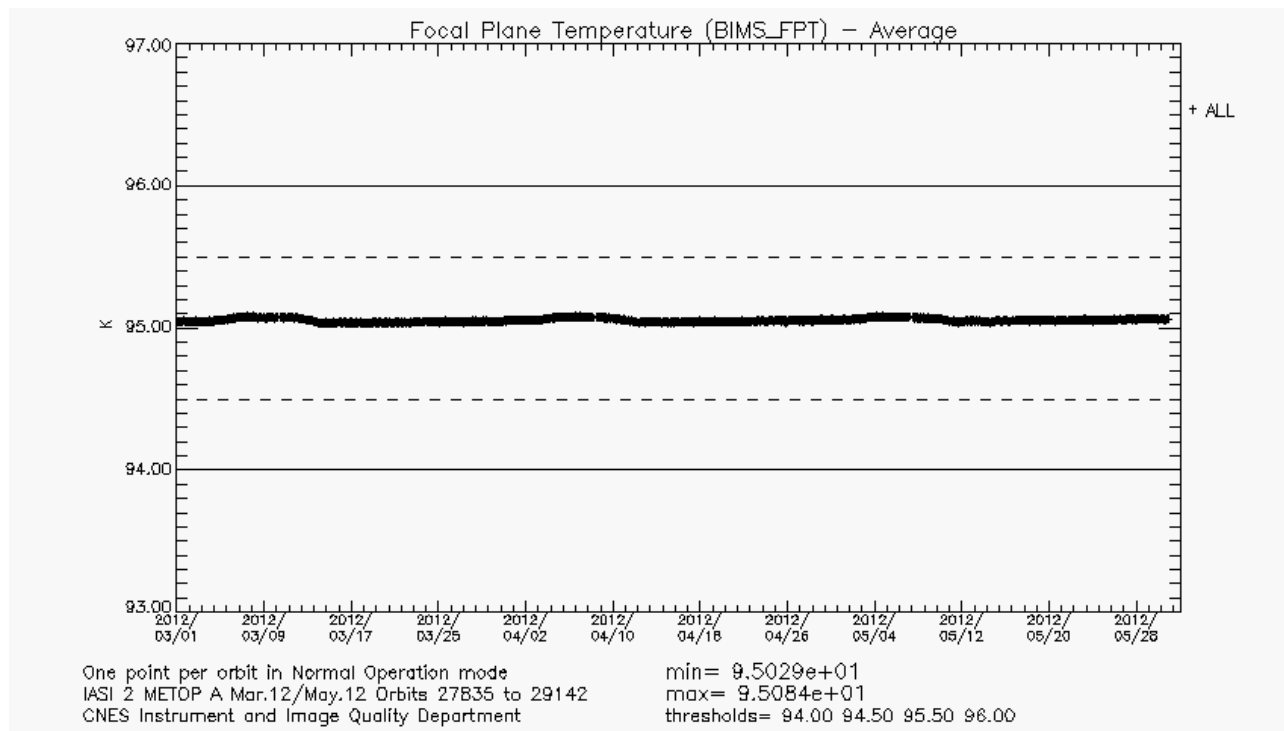
Figure 21 : Focal Plane Temperature
