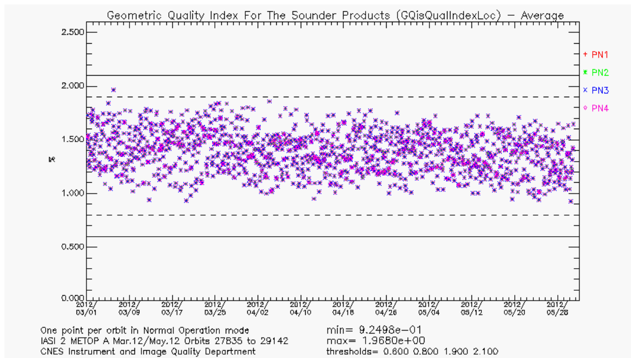
Figure 13 : GQisQualIndexLoc average (LI data index for ground localisation quality)
