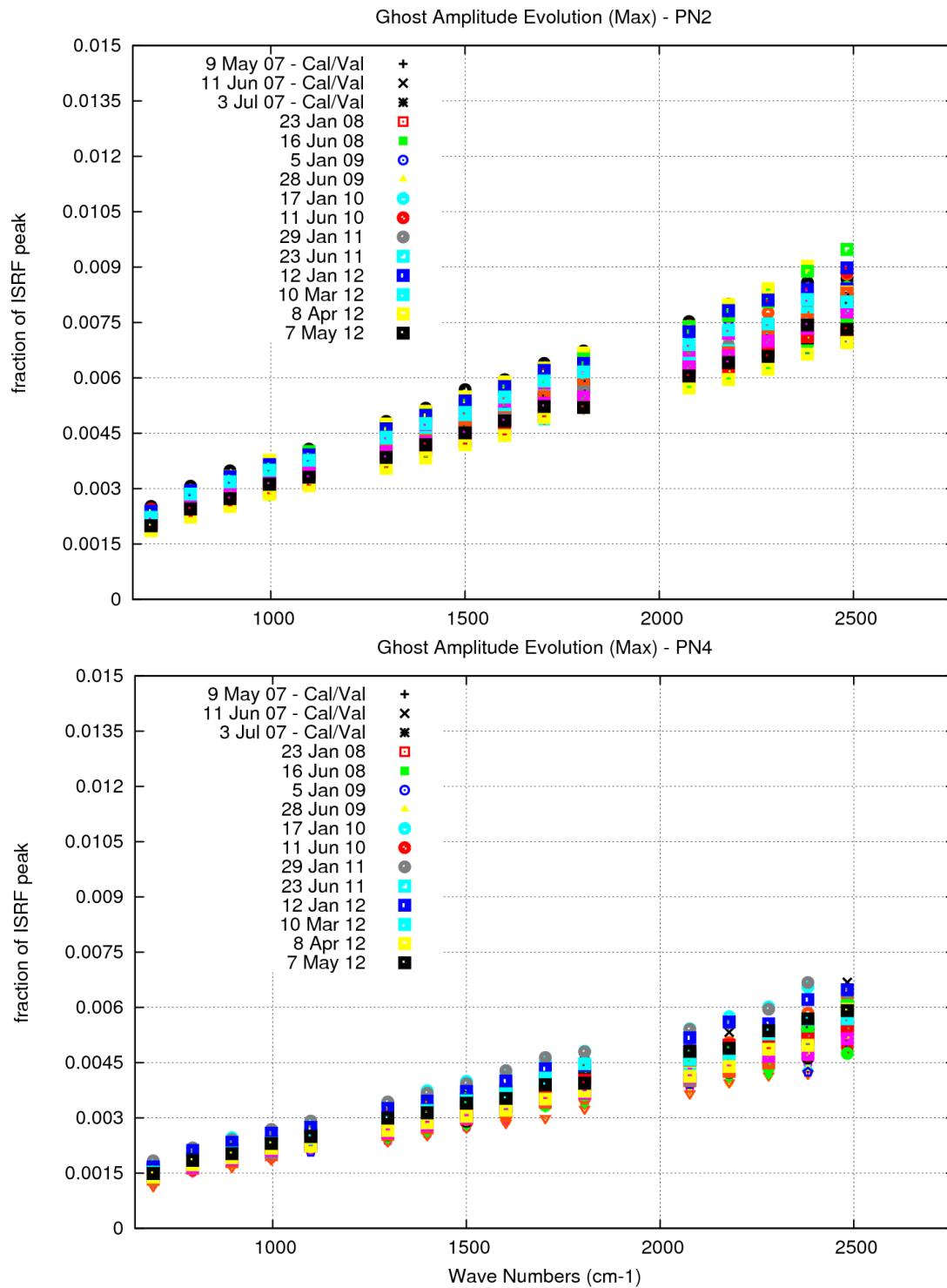
Figure 28 : Ghost amplitude as a function of wave number for different time (Top: pixel 2, bottom: pixel 4)
