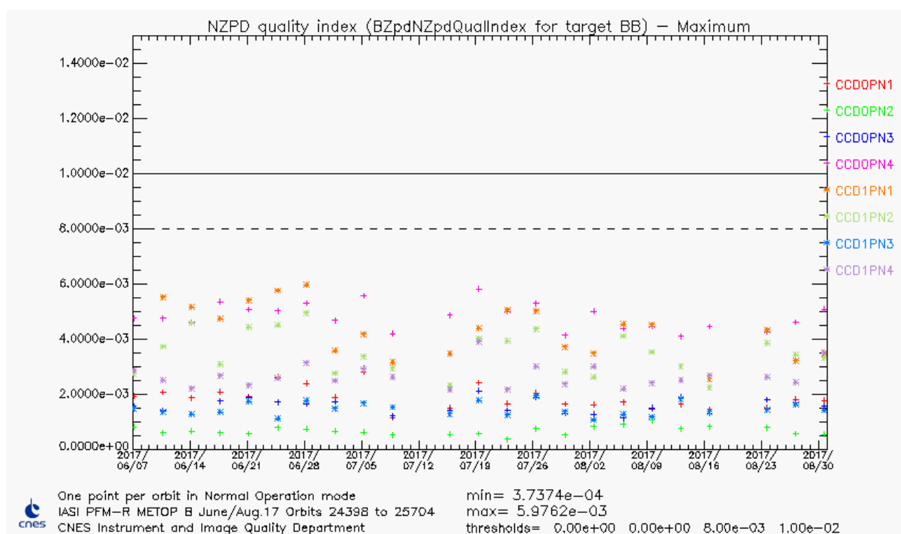
Figure 10 : Max of NZPD quality index for all pixels and CCD - BB
