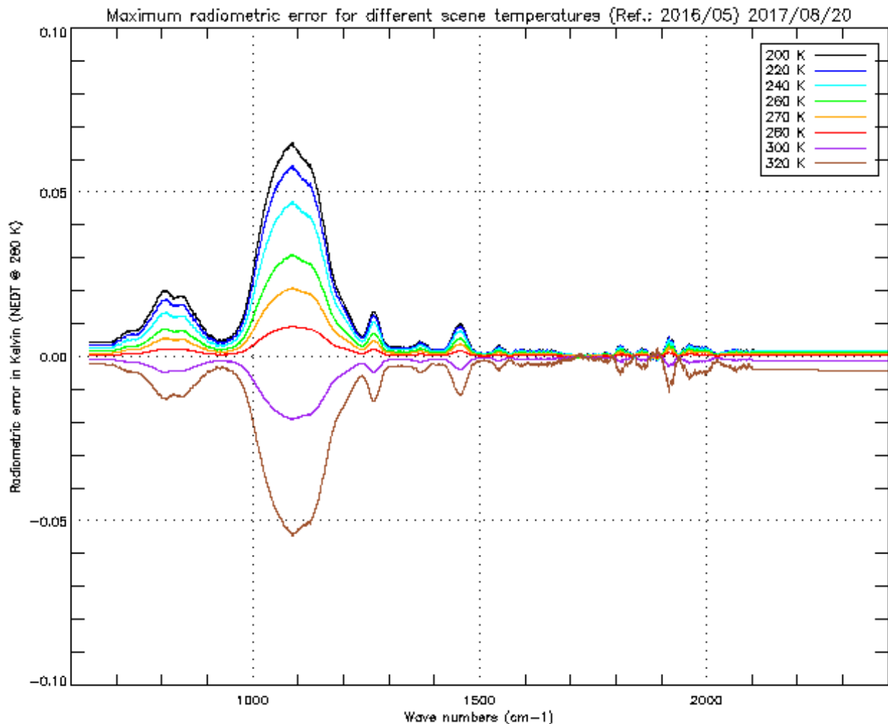
Figure 23 : Radiometric calibration error due to scan mirror reflectivity dependency with viewing angle Maximum effect on SN1 for different scene temperature. Done with the period May 16 / August. 17
