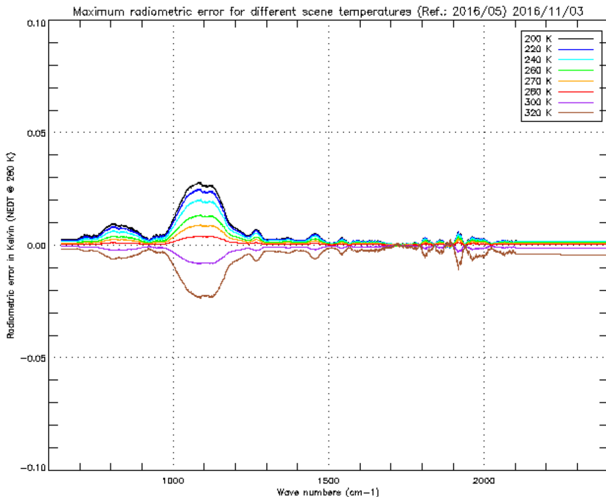
Figure 22 : Radiometric calibration error due to scan mirror reflectivity dependency with viewing angle Maximum effect on SN1 for different scene temperature. Done with the period May / Nov. 16
