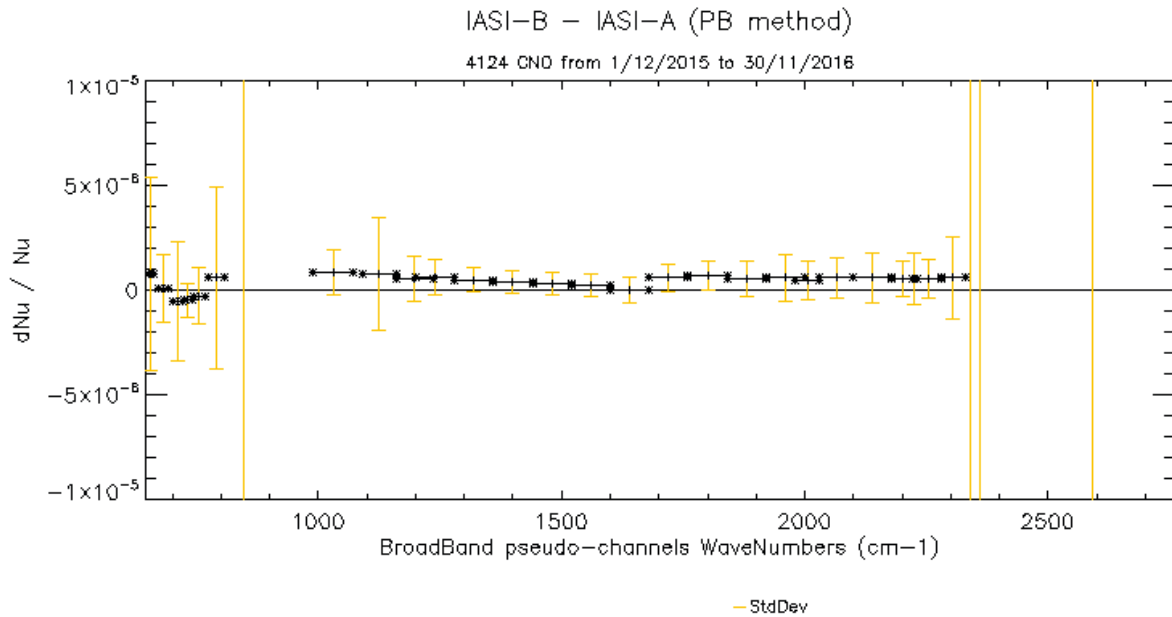
Figure 39 : Mean (black curve) and standard deviation (yellow curve) of the difference spectral calibration \Delta\nu/\nu between IASI-B and A.
