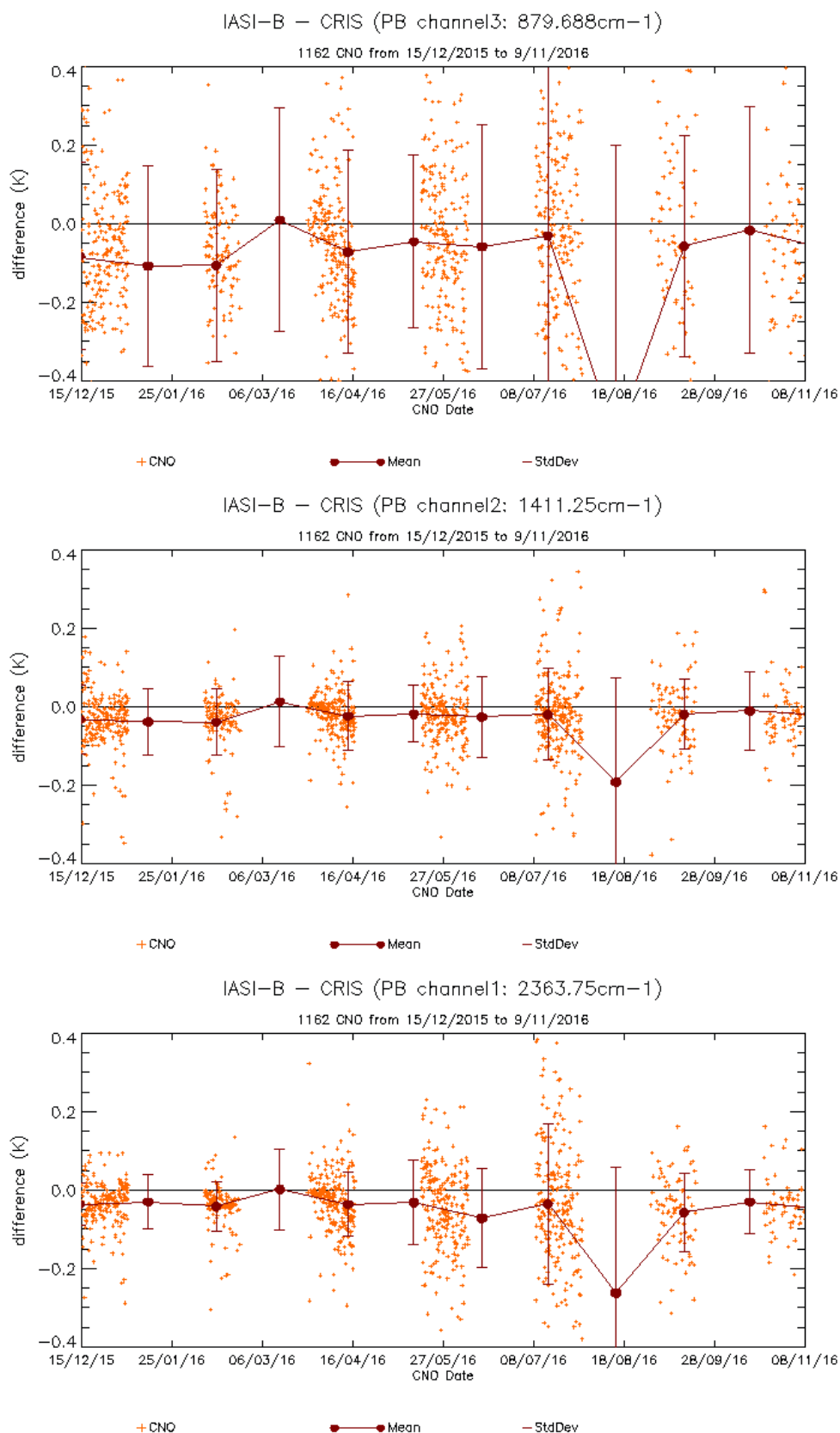
Figure 42 : Temporal evolution of the differences IASI-B – CRIS in brightness temperature over the approximate three IASI bands, with monthly means.
