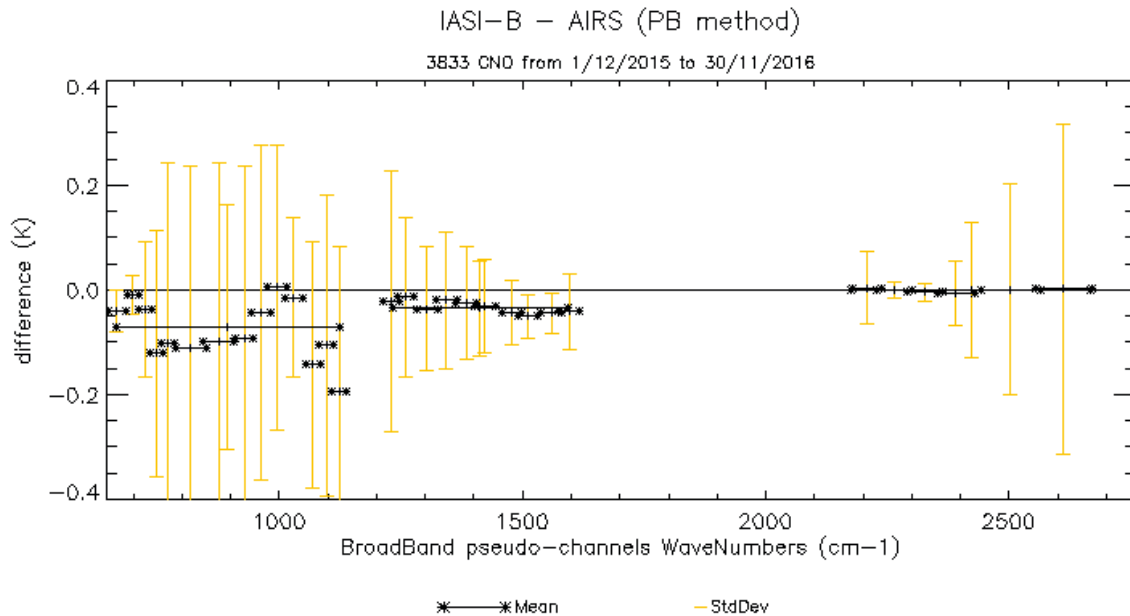
Figure 43 : Mean (black curve) and standard deviation (yellow) of the difference in brightness temperature IASI-B – AIRS.
