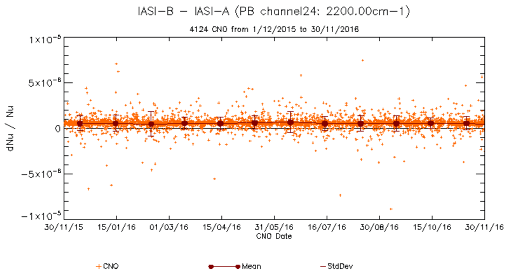
Figure 40 : Temporal evolution of the difference spectral calibration \Delta\nu/\nu between IASI-B and A in the spectral window centered around 2200cm-1.
