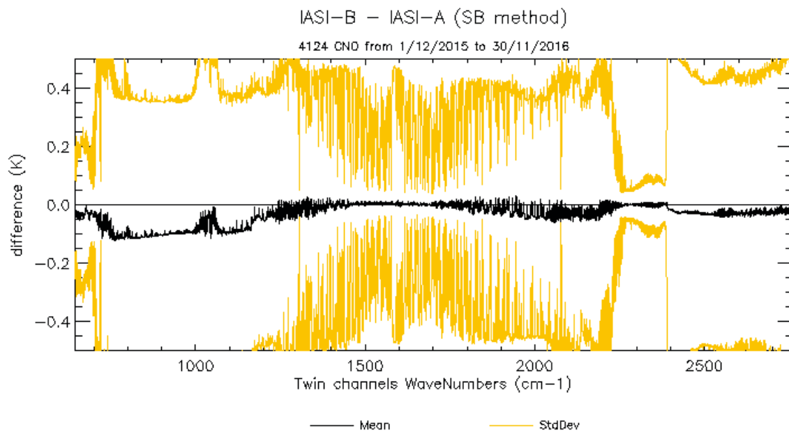
Figure 37 : Mean (black curve) and standard deviation (yellow) of the difference in brightness temperature IASI-B – IASI-A
