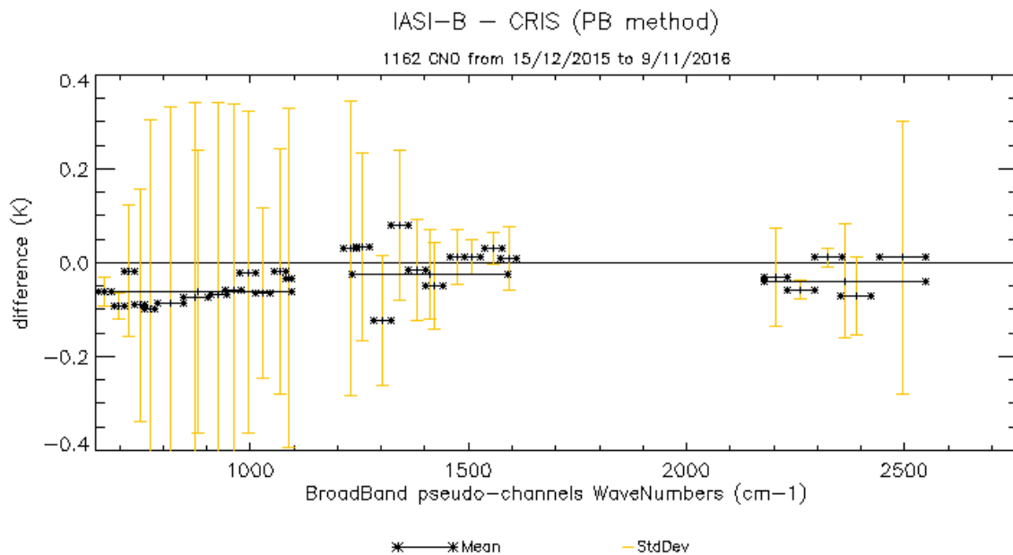
Figure 41 : Mean (black curve) and standard deviation (yellow) of the difference in brightness temperature IASI-B – CRIS
