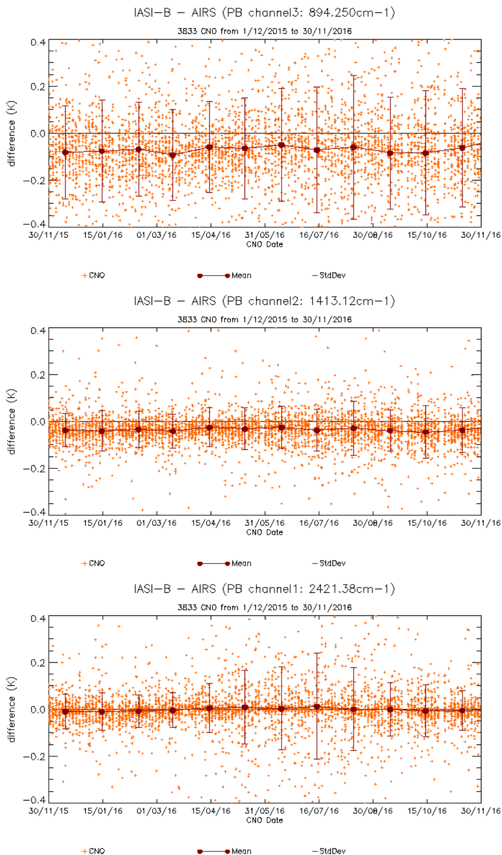
Figure 44 : Temporal evolution of the differences IASI-B - AIRS in brightness temperature over the approximate three IASI bands, with monthly mean.
