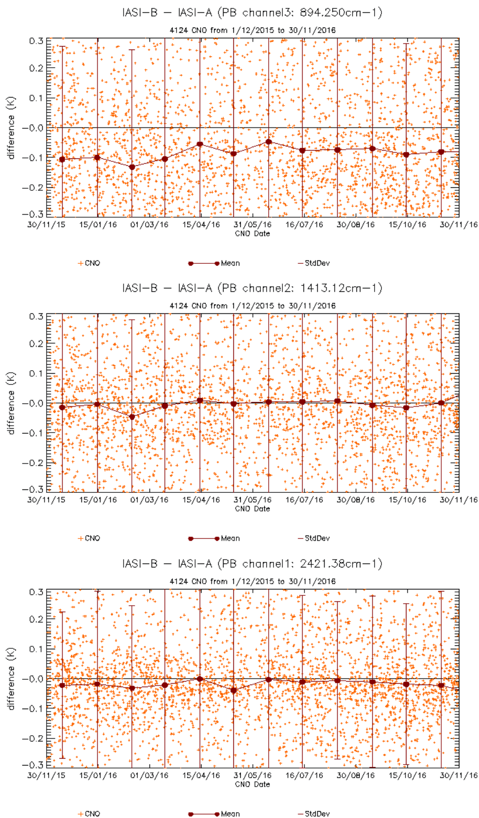
Figure 38 : Temporal evolution of differences IASI-B – IASI-A in brightness temperature spectrally integrated over the approximate three IASI bands
