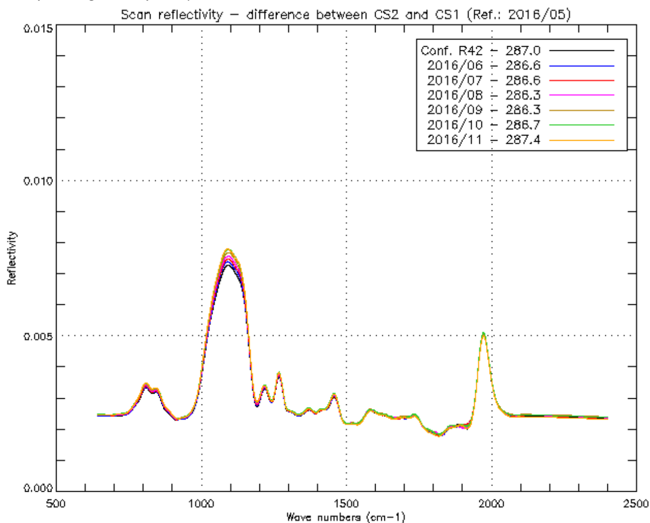
Figure 21 : Scan mirror reflectivity evolution
