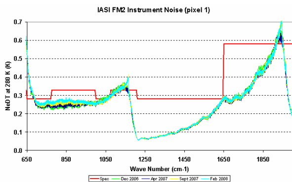
Fig. 2: FM2 instrument noise (NEdT @280K) between December 2006 and March 2008
