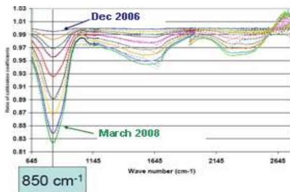
Fig. 3: FM2 transmission loss due to ice contamination
